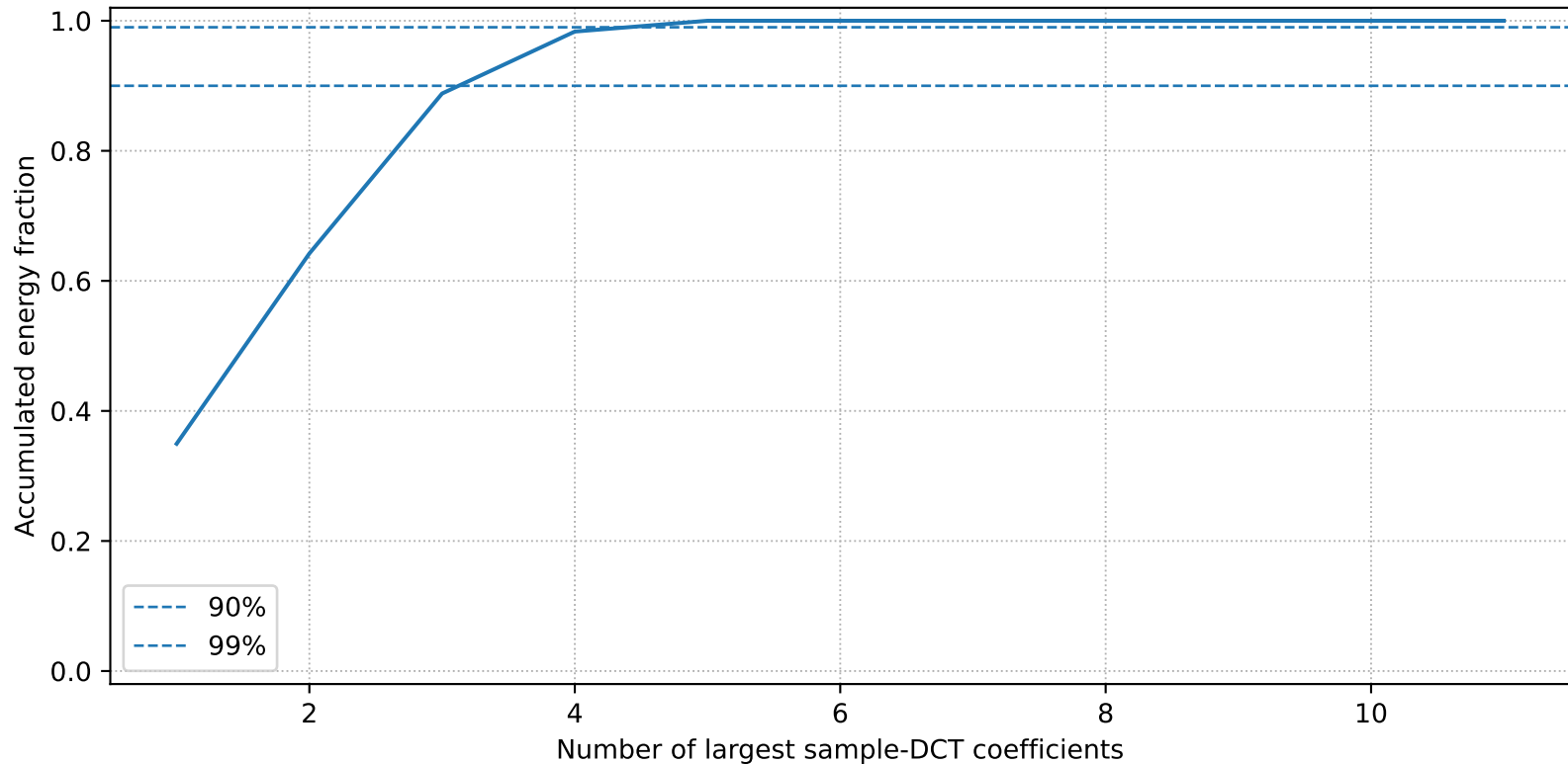
Compressibility of x[n] in DCT domain
