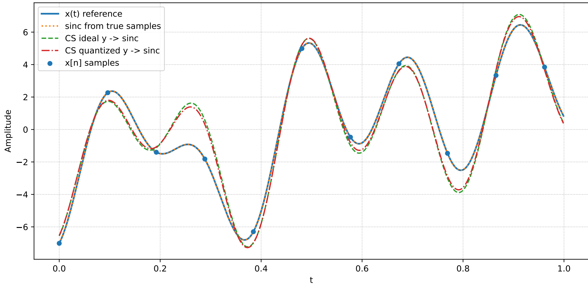
CS + FDMA debug: x(t) , x[n] , CS recovery, sinc reconstruction
