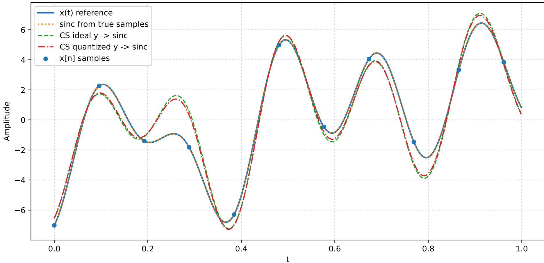
CS + FDMA debug: x(t) , x[n] , CS recovery, sinc reconstruction
