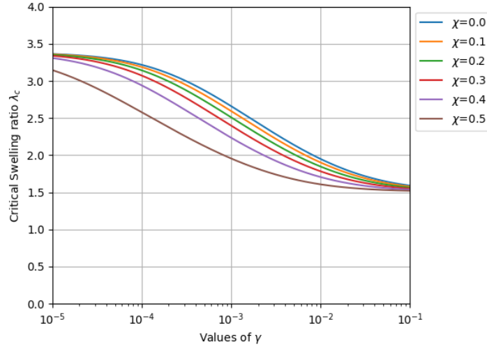
Figure 3: Critical swelling ratio
