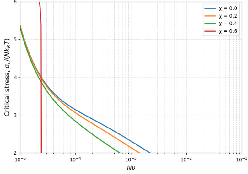
Figure 6: Critical compressive stress
