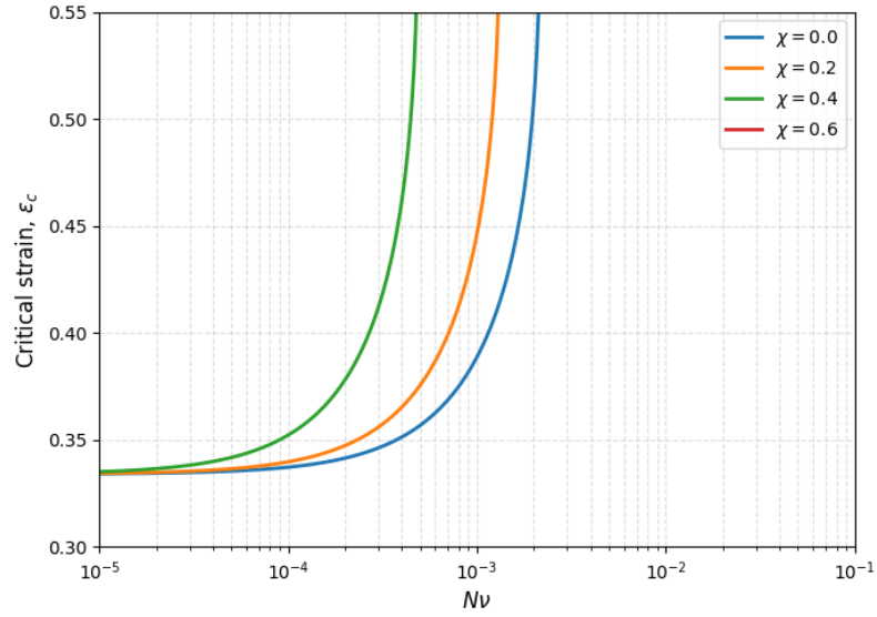
Figure 7: Critical strain
