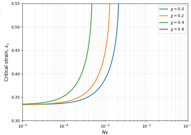
Figure 7: Critical strain
