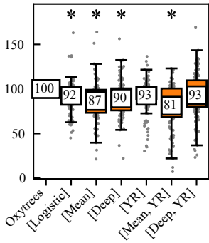
Inductive | PMP = 0% | AUPRC
