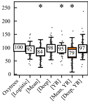
Inductive | PMP = 50% | AUPRC
