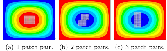
Figure 7: Model validation of the optimization for the first vibration mode using up to 3 patch pairs applied to the plate.
