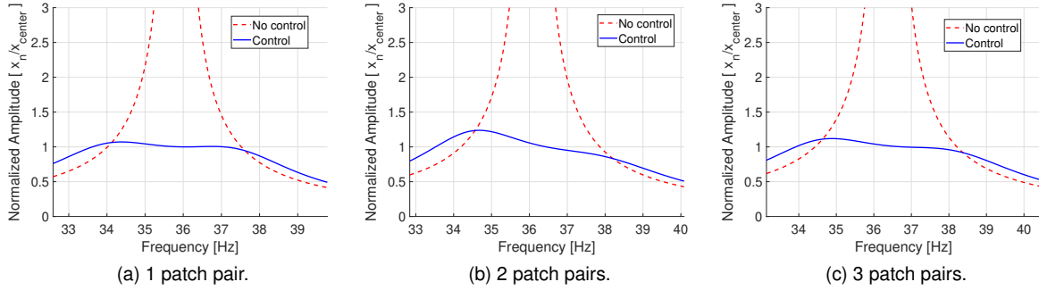
Figure 4.4: Harmonic solutions for the 1st vibration mode using a single shunt circuit with calibrated RL values.
