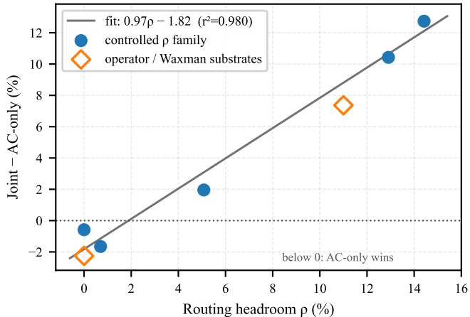
(b) the routing-headroom law
