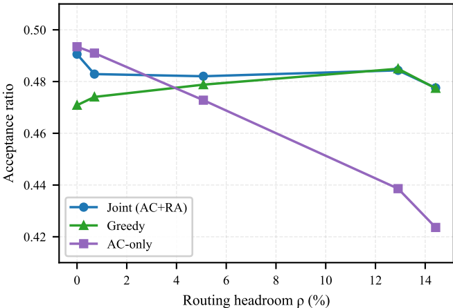
(a) policies as routing headroom grows
