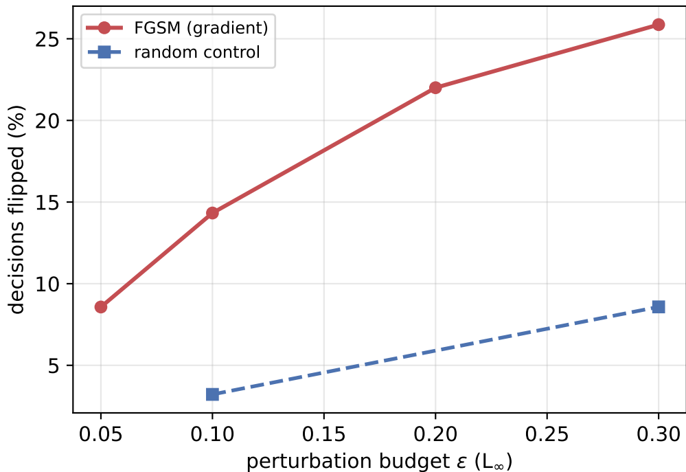
FGSM reliably flips routing decisions (CC-Simple, 2× hotspot)
