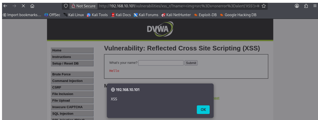
Figure 25: screenshots/2026-08-12/entrada22-xss-reflected-medium-img-bypass.png
