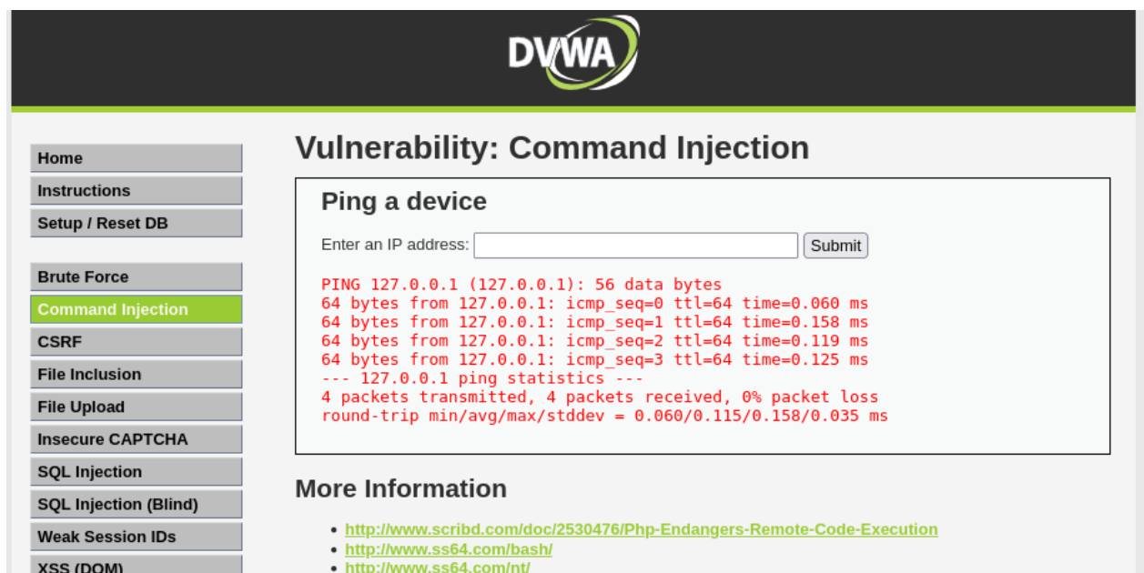
Figure 12: screenshots/2026-08-12/entrada18-cmdinjection-medium-semicolon-filtrado.png
