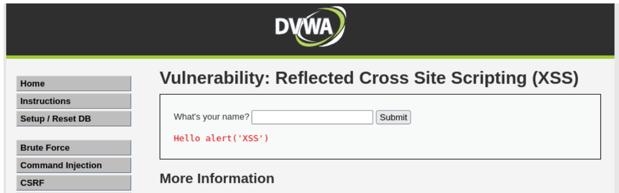
Figure 24: screenshots/2026-08-12/entrada22-xss-reflected-medium-script-filtrado.png
