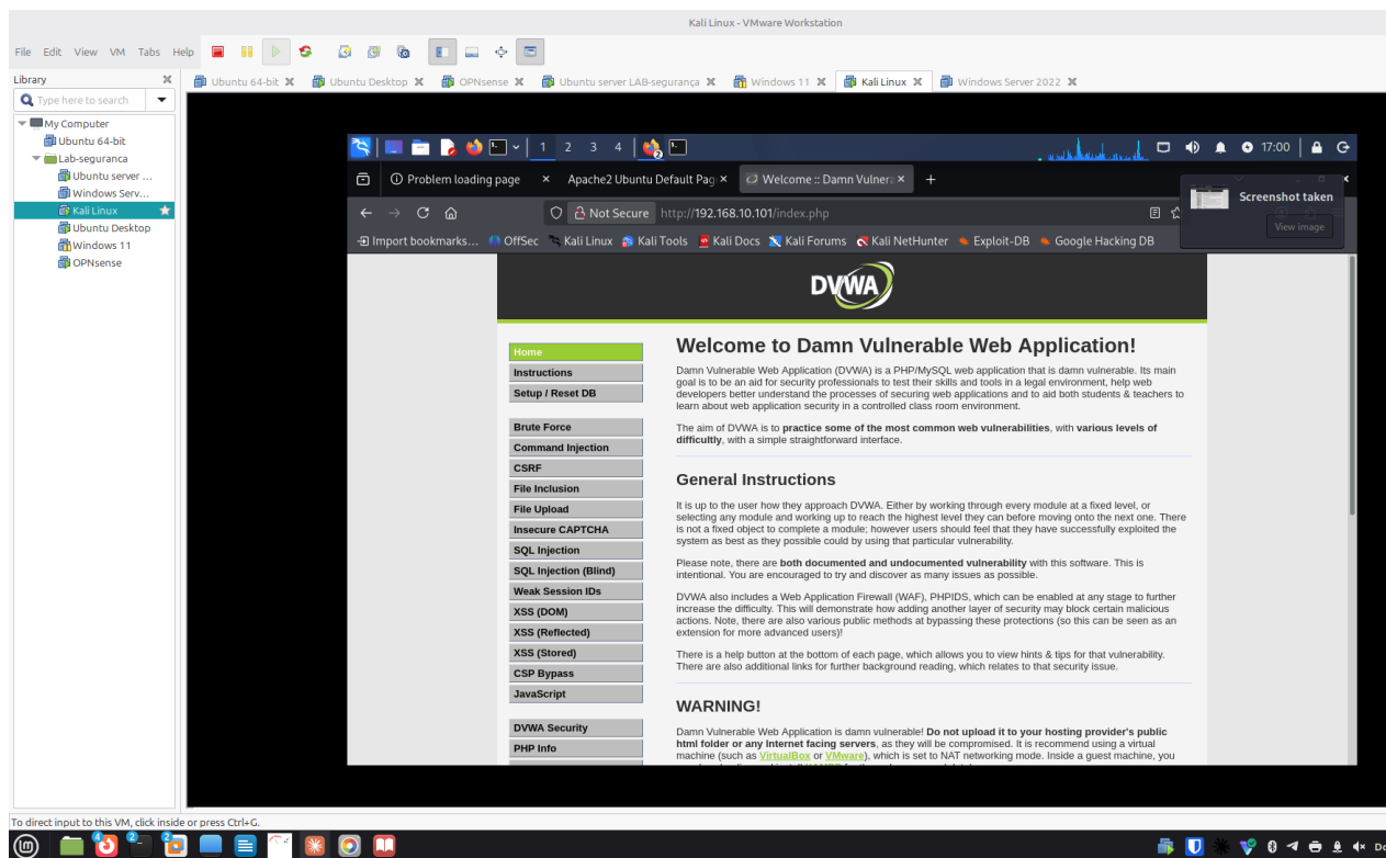
Figure 2: screenshots/2026-08-02/entrada07-dvwa-welcome-page.png
