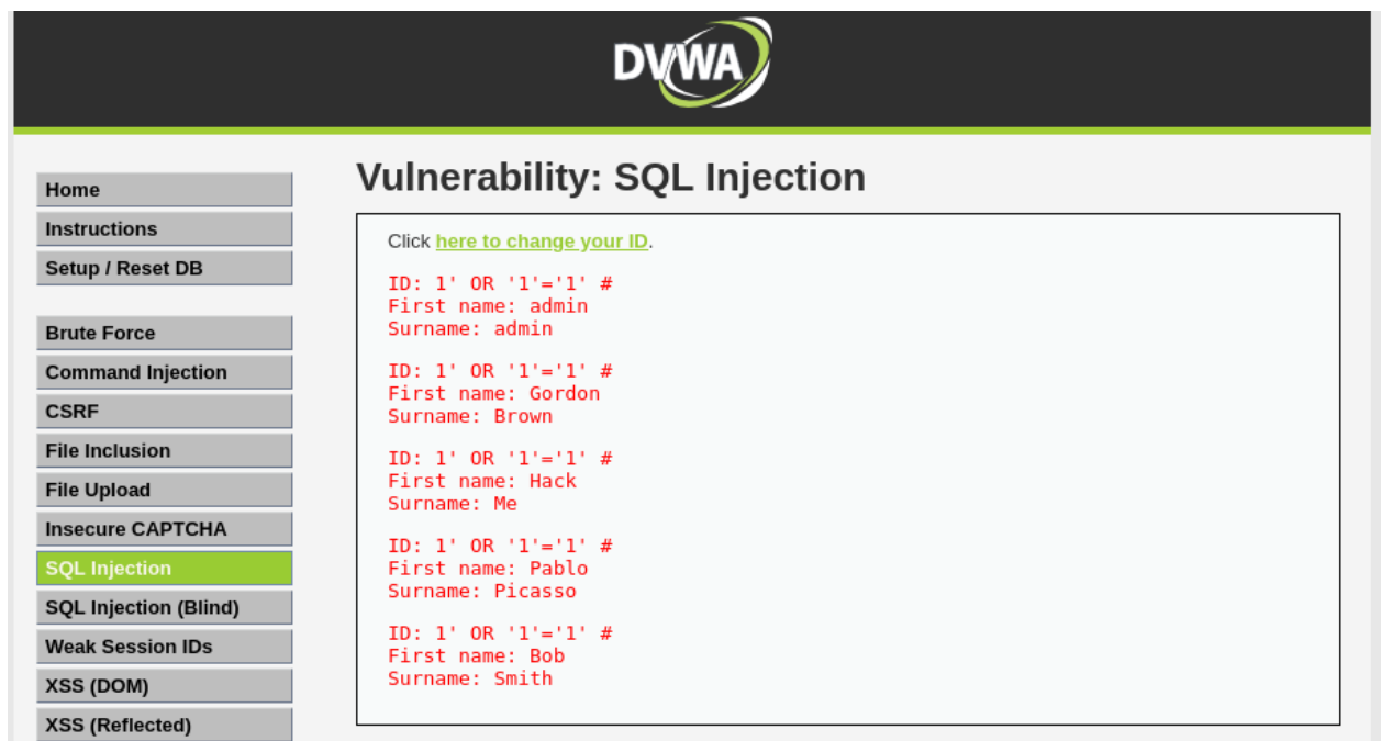
Figure 7: screenshots/2026-08-11/entrada15-sqli-high-5-utilizadores.png
