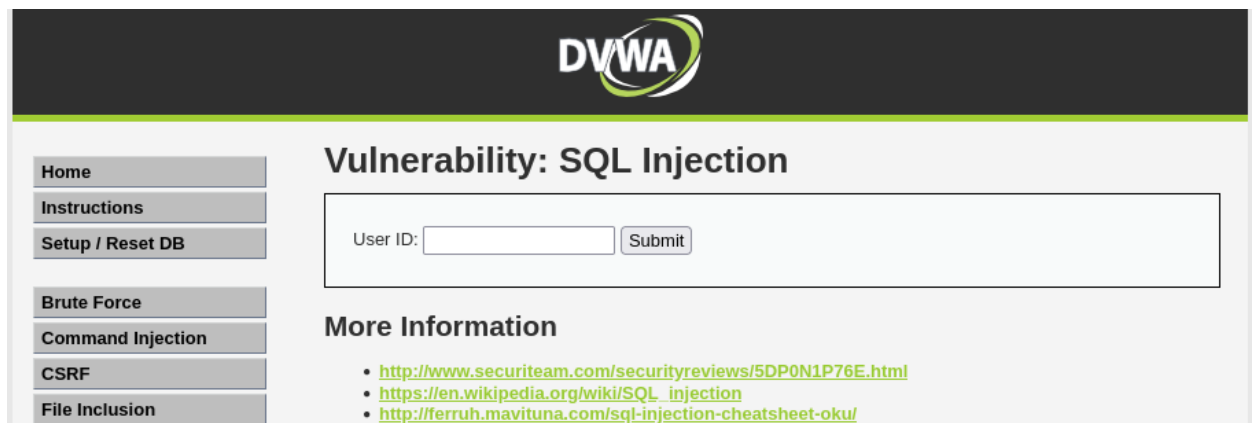
Figure 8: screenshots/2026-08-12/entrada16-sqli-impossible-ataque-falhado.png
