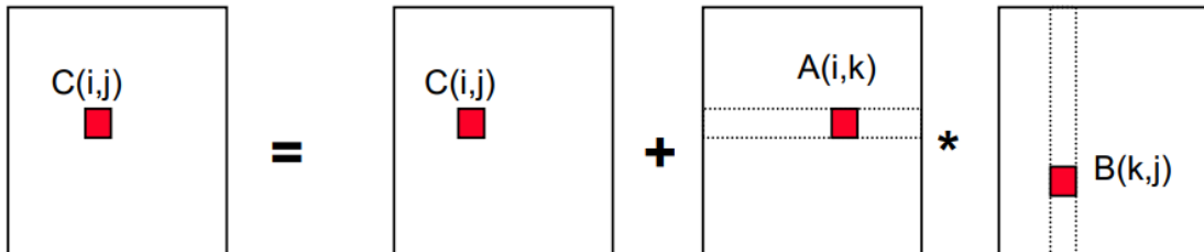
Figure 3.4: Blocked matrix multiplication algorithm.
