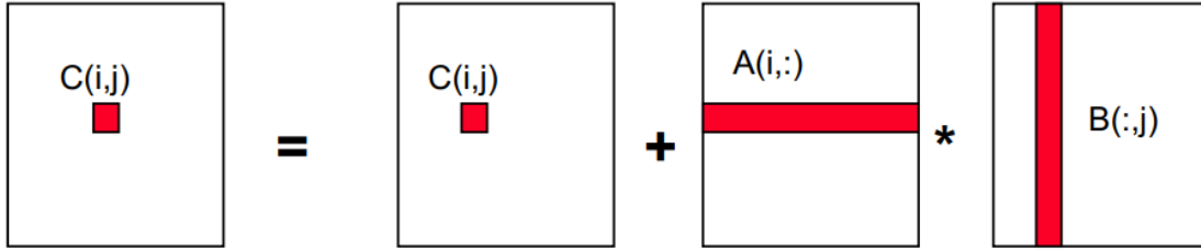
Figure 3.3: Naive matrix multiplication algorithm.
