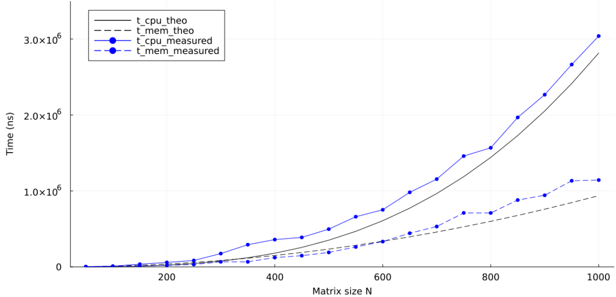
Figure 3.10: FP32 MxM: theoretical vs. measured times. t_{\text{CPU}} scales as O(N^3) and dominates for moderate/large N ; measured time tracks the compute-bound model thanks to cache-blocked reuse. t_{\text{mem}} is a lower bound assuming RAM-limited traffic; real runs reuse data from caches and remain above it.
