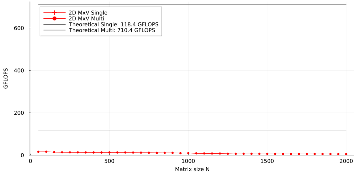
Figure 8.7: Float32 2D Laplacian (looped MxV): single vs. multi-threaded performance.
