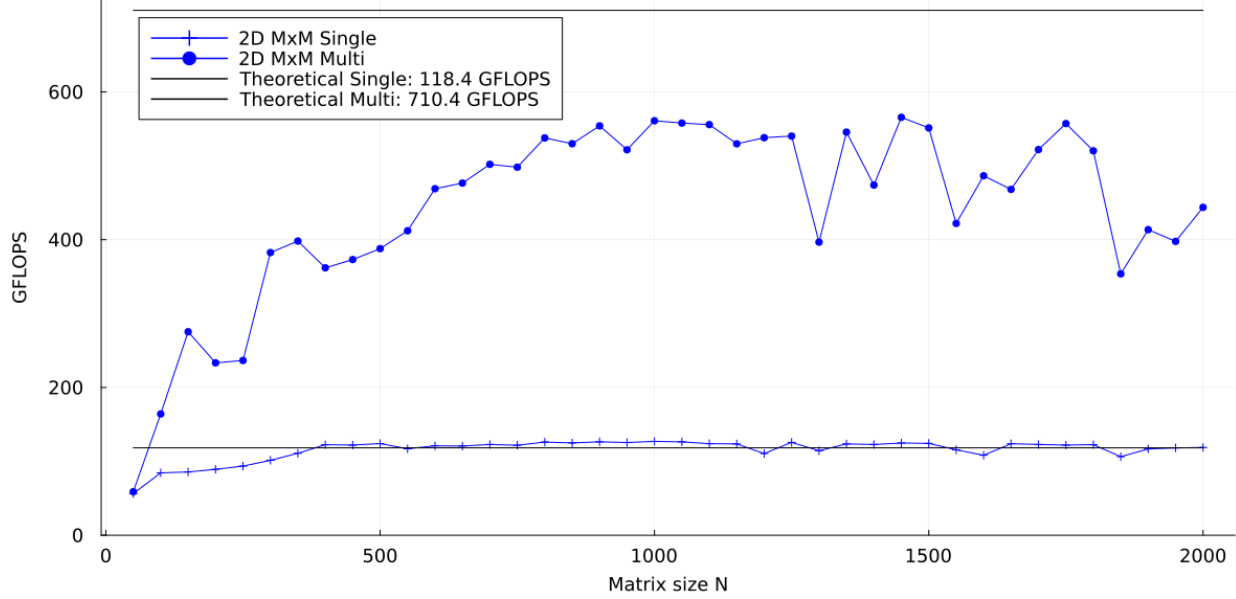
Figure 8.4: Float32 2D Laplacian (MxM): single vs. multi-threaded performance.
