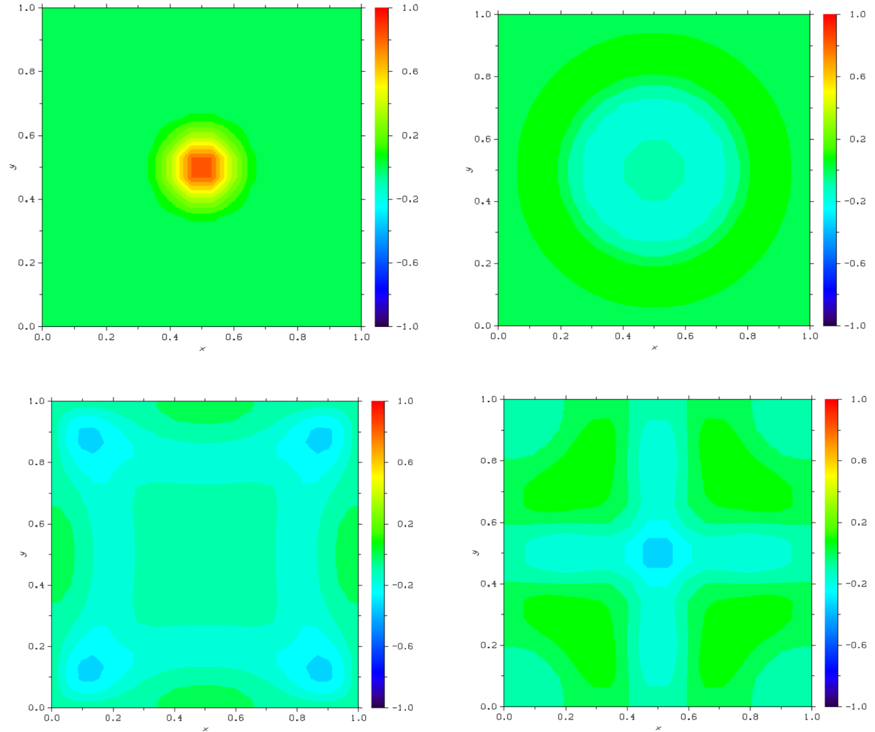
Figure 8.10: 2D Wave Equation Evolution. Numerical solution of the 2D wave equation implemented in NumericalHub and visualized using the plot_contour function.
