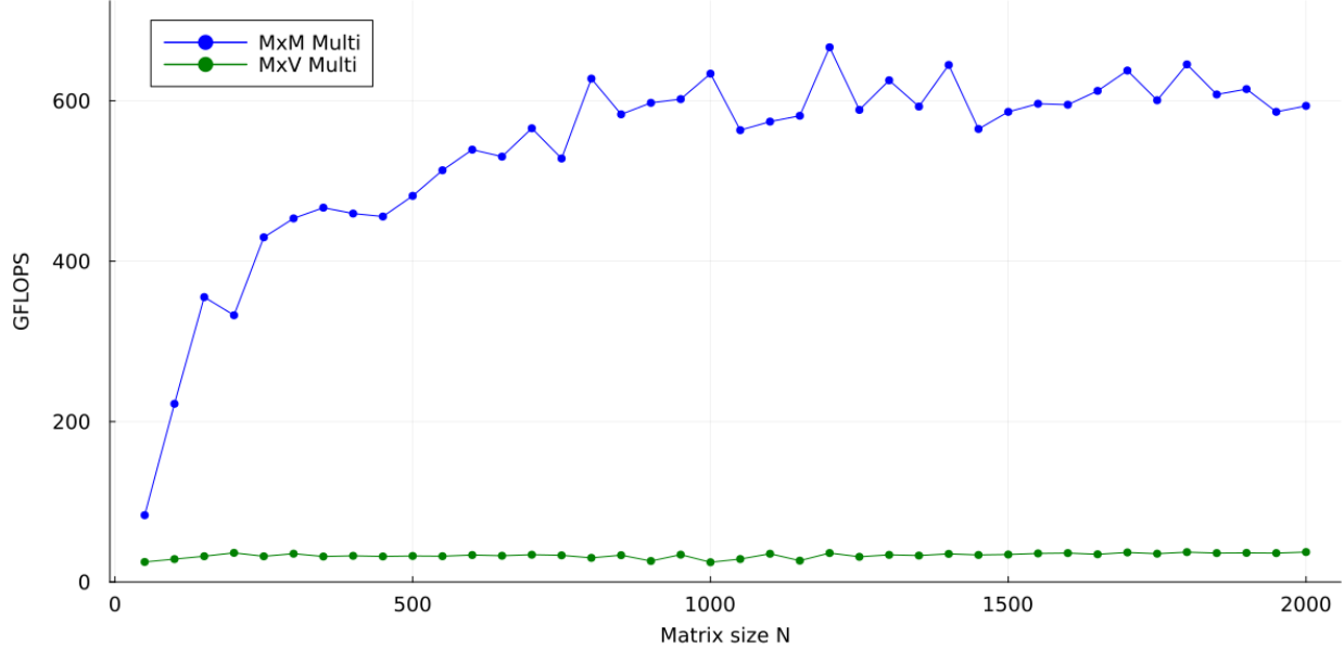
Figure 3.6: FP32, multi-core: MxM vs. MxV. MxM gains markedly from parallelism once N is sufficient to amortize threading overheads and feed all cores; MxV barely scales because RAM bandwidth is shared and already constraining performance, so extra cores cannot increase sustained FLOPS meaningfully.
