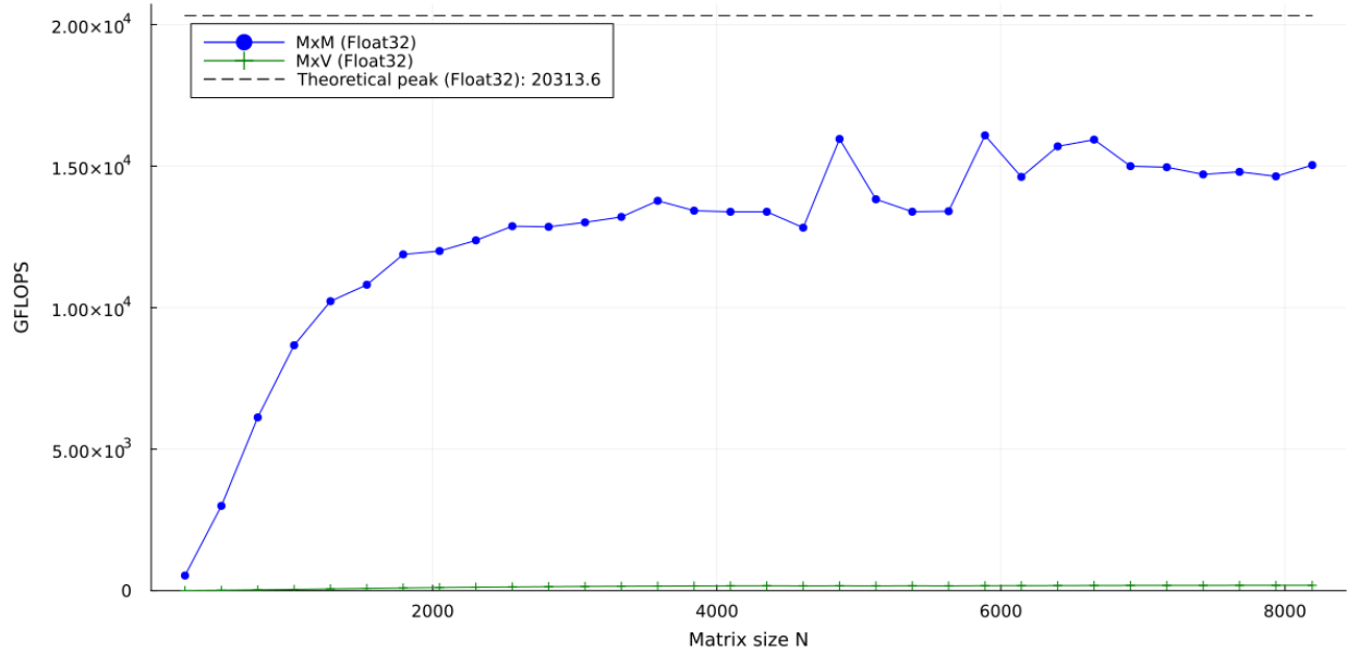
Figure 4.3: GFLOPS GPU FP32: MxM vs. MxV. MxM, being compute-bound, climbs sharply and approaches a high plateau as cuBLAS tiles reuse data in shared memory and L2 cache. On the other hand, MxV, being memory-bound, sits much lower and changes little with N : extra parallelism cannot overcome the memory wall, so GFLOPS remain well below MxM.
