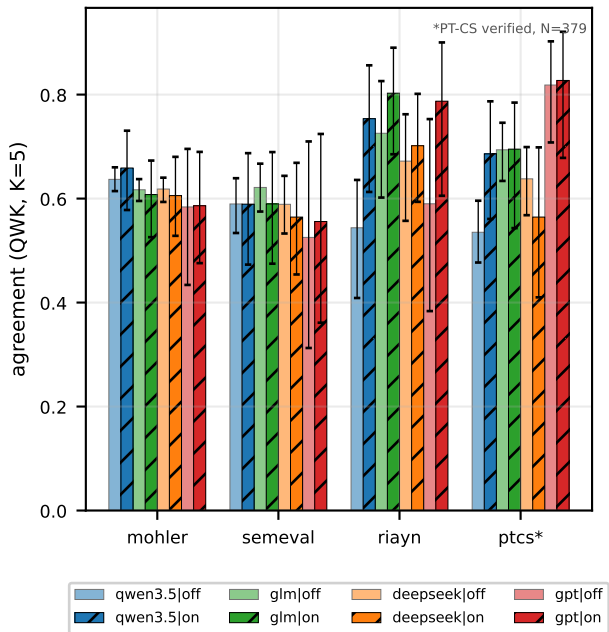
RQ4: agreement by model \times reasoning, per dataset
