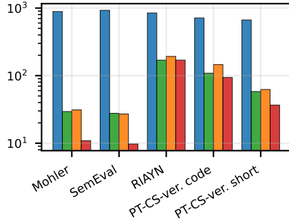
cost: ON/OFF token premium ( \times , log)
