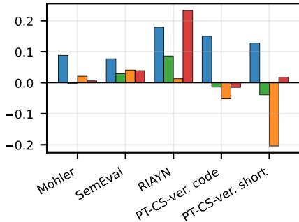
agreement: \Delta QWK (above 0 = reasoning helps)
