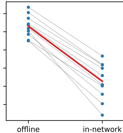
LightGBM
