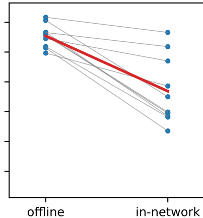
XGBoost
