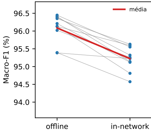
RF
