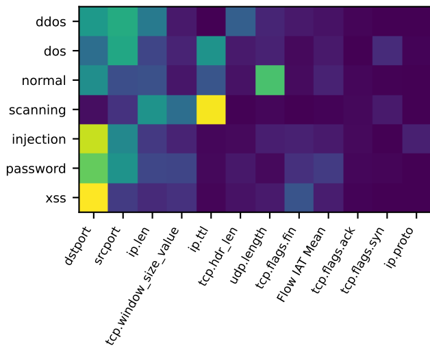
LightGBM
