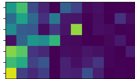
XGBoost
