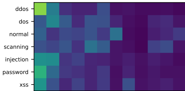
RF
