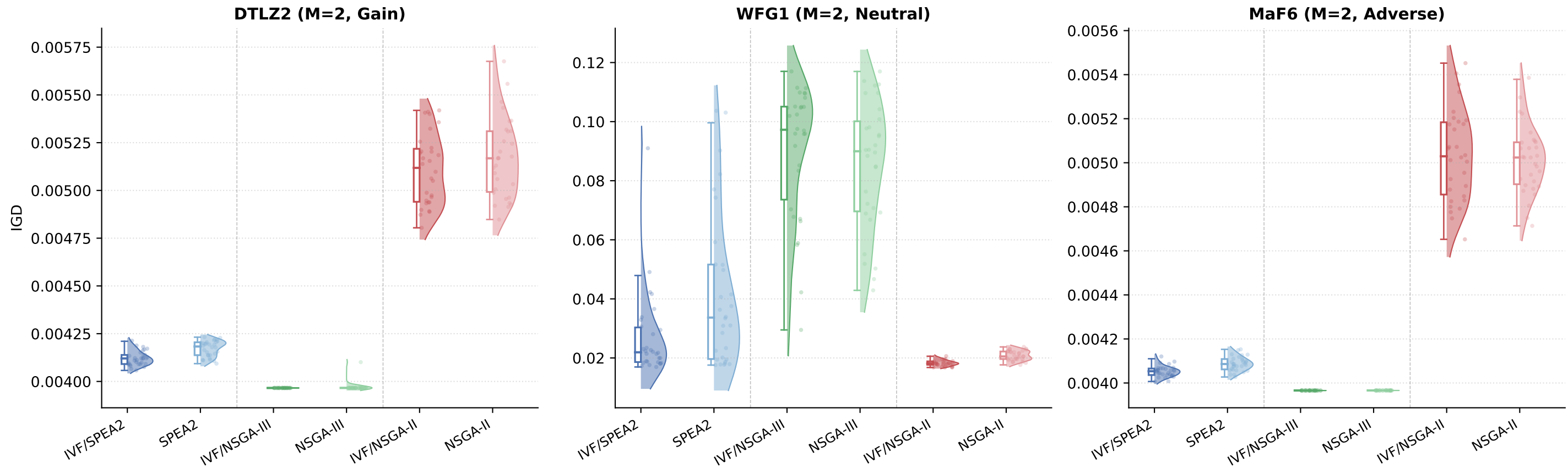
IGD distributions across algorithms: representative M=2 instances
