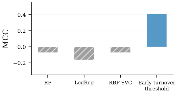
(b) MCC
