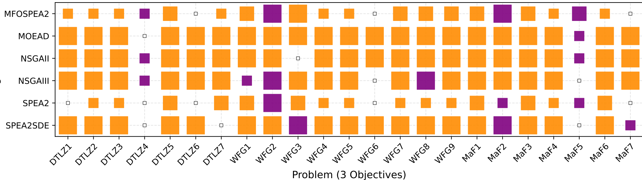
Performance vs. IVFSPEA2
