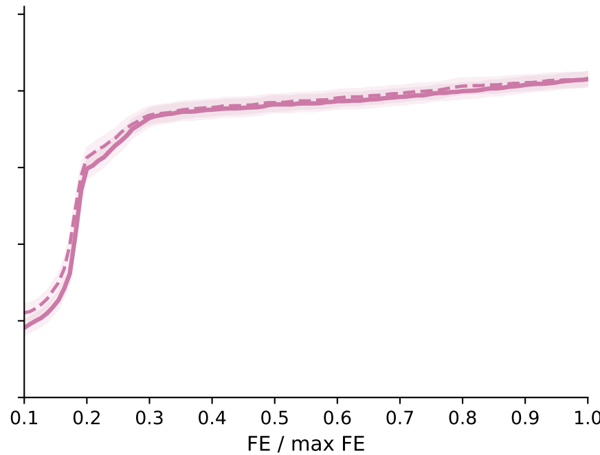
IVF/NSGA-III
