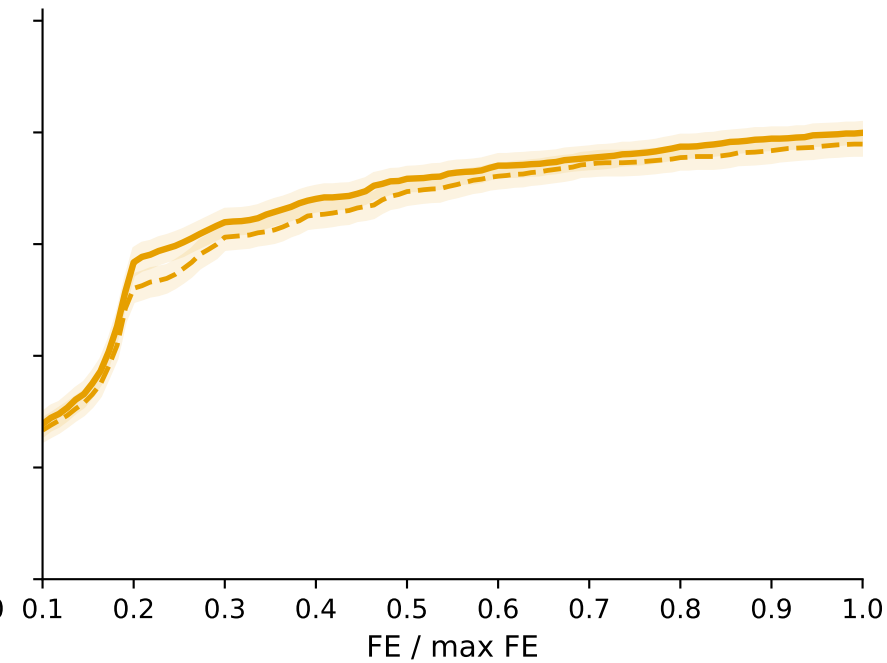
IVF/NSGA-II
