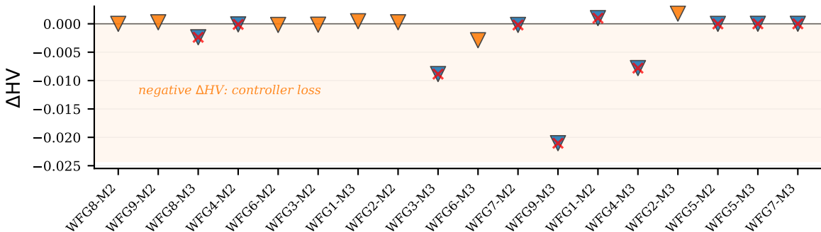
(b) Controller \Delta HV in WFG instances
