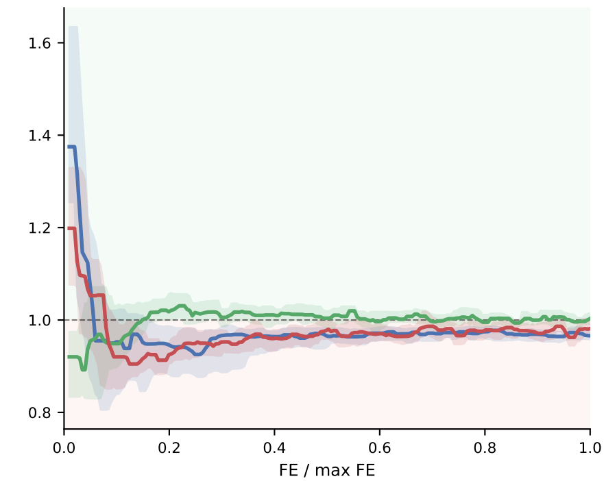
WFG2 ( M = 2 )
