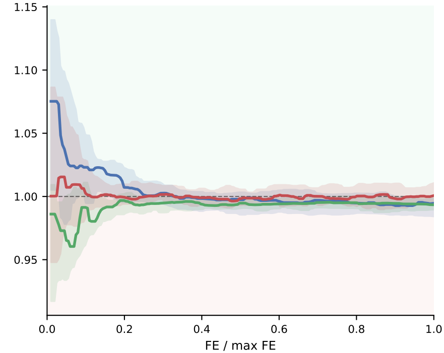
WFG2 ( M = 2 )
