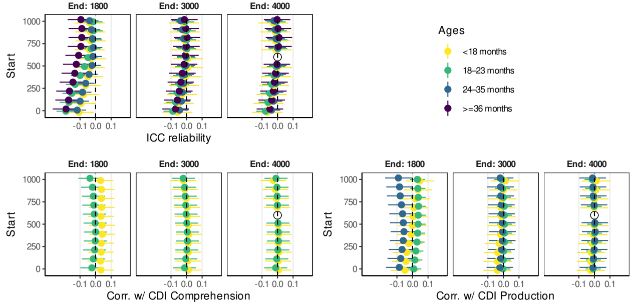
Figure S5: Model results split out by age comparing the effects different accuracy windows to the index length of 600–4000 ms for different dependent variables.
