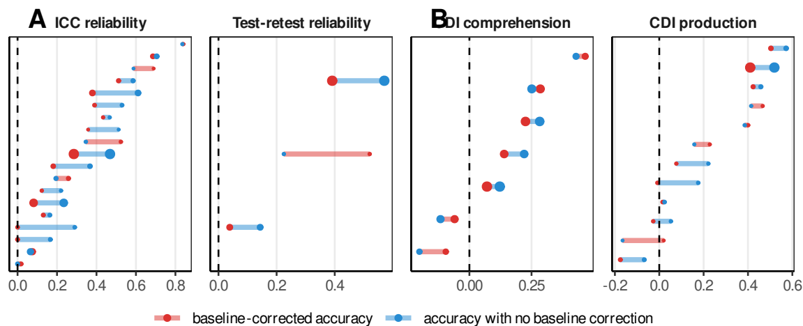
Figure S6: Comparison between a baseline-corrected accuracy in red and accuracy in blue across datasets and measures. Both use a post-stimulus window of 300 - 1800ms, the baseline window was -2000 - 0ms.
