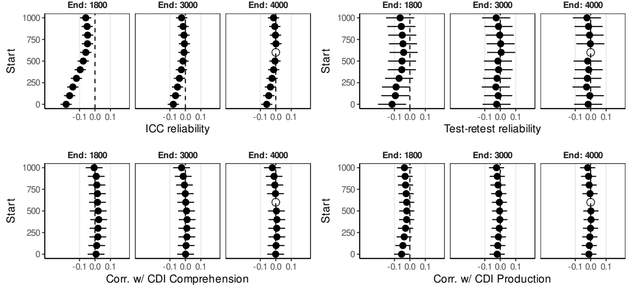
Figure S4: Model results comparing the effects different accuracy windows to the index length of 600–4000 ms for different dependent variables.
