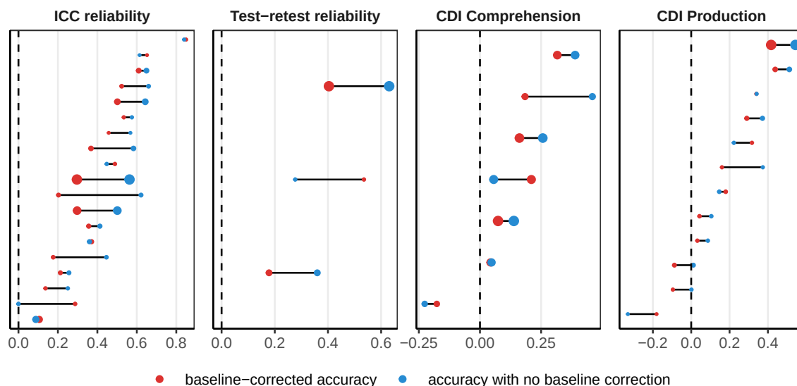
Figure 3. Comparison between a baseline-corrected accuracy in red and accuracy in blue across datasets and measures. Both use an accuracy window of 600 - 4000ms, the baseline window was -2000 - 0ms.
