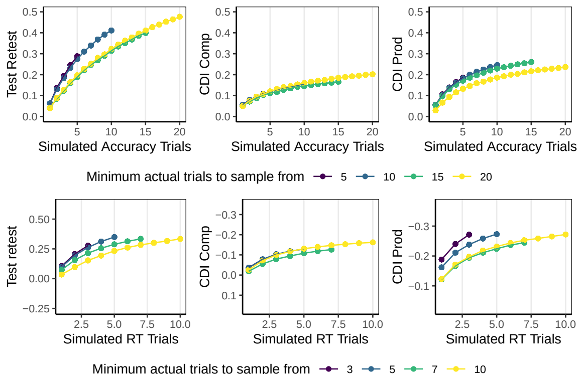
Figure 7. Simulations of measurement properties for different trial counts, created by downsampling trials for all children with different trial minimums. Shown for an accuracy window of 600 to 4000 ms with no trial- or administration- level exclusions.
