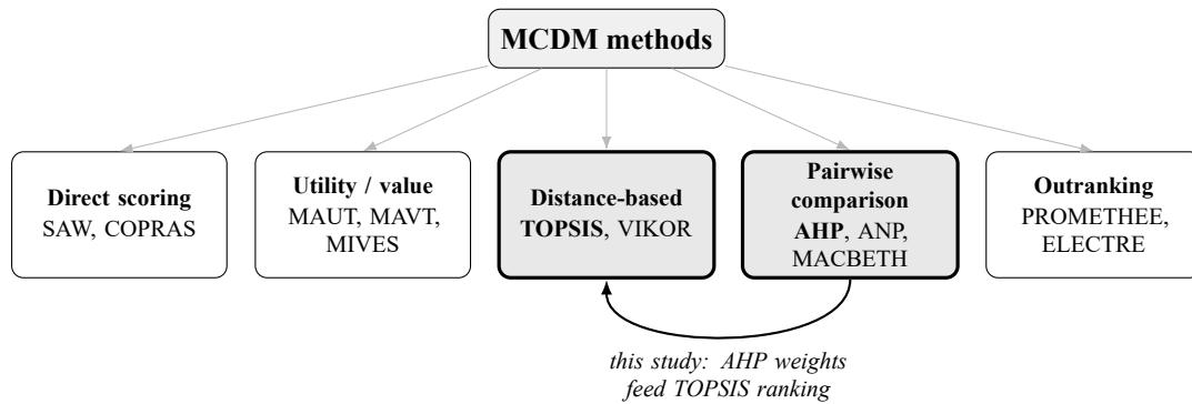
Figure 2.1: The five families of MCDM methods, with the pairwise-comparison and distance-based groups combined in this study.
