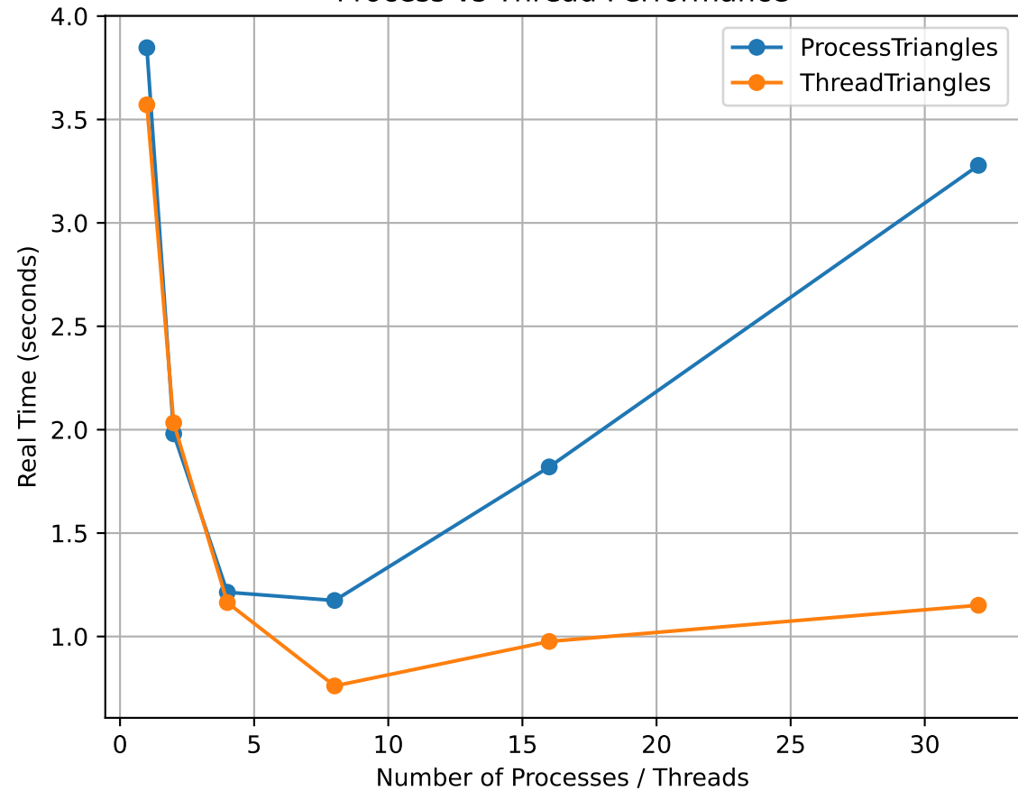
Process vs Thread Performance
