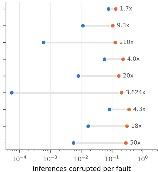
CIFAR-100
