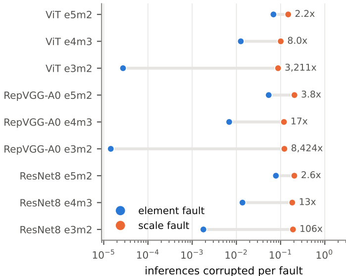
CIFAR-10
