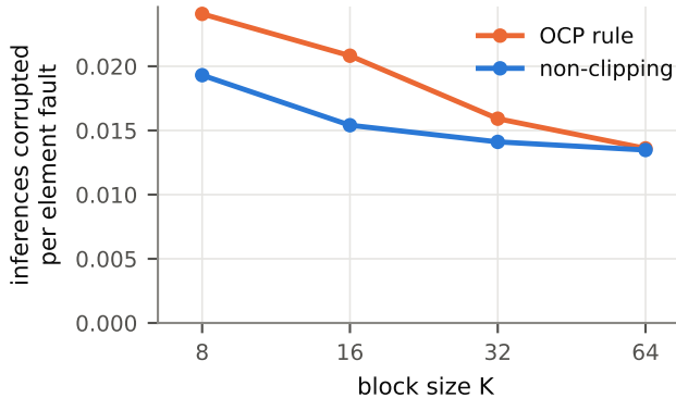
ResNet8, e4m3
