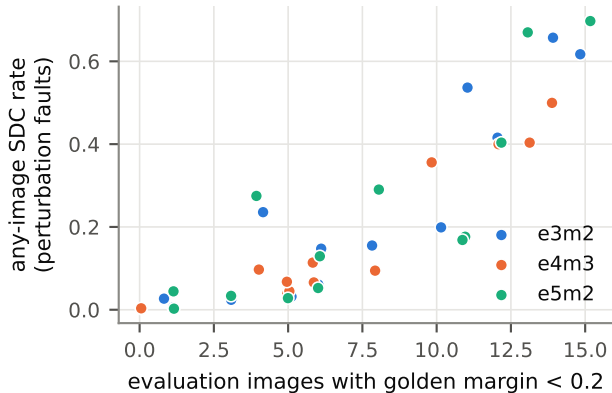
The any-image rate counts near-ties (39 networks, Spearman +0.89)
