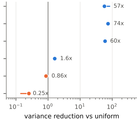
ResNet8, e4m3
