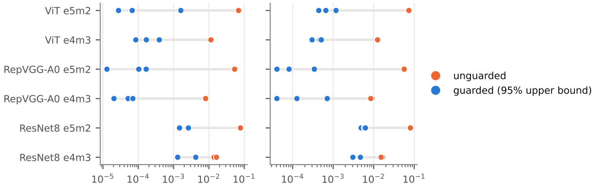
CIFAR-10
