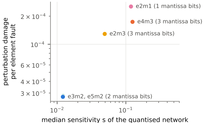
(b) sensitivity, not mantissa width, tracks perturbation damage (ViT)
