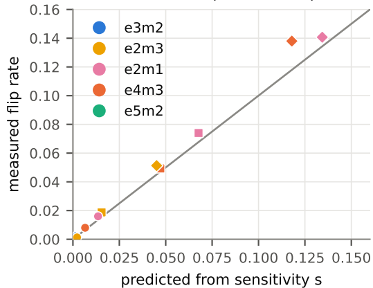
(a) probe: one weight moved by 0.5 / 1.5 / 3 rms ( r = +0.998 )
