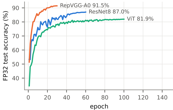
CIFAR-10
