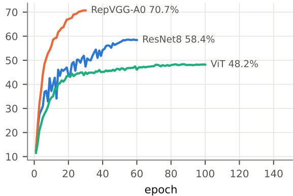
CIFAR-100
