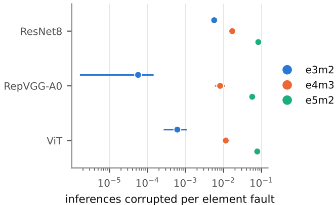
CIFAR-100
