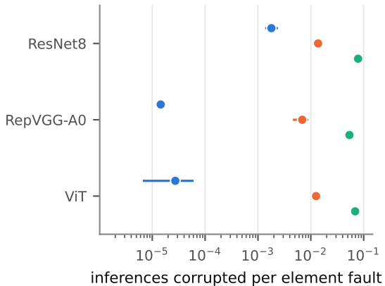
CIFAR-10
