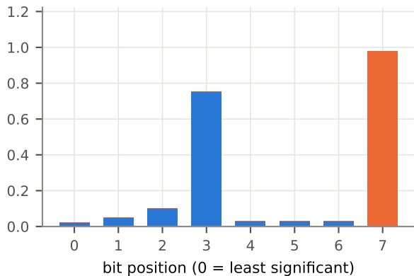
shared E8M0 scale
