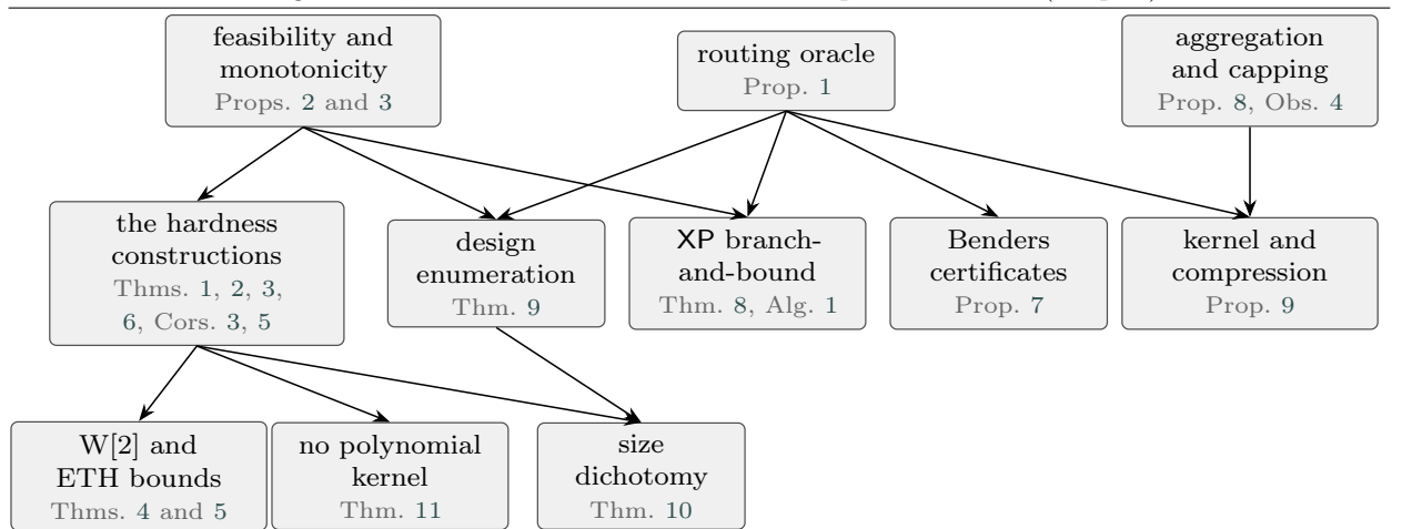
Figure 8 The results of the paper as a diagram, each box naming its numbered statements. A solid arrow points from a result to one whose proof uses it, and no other relation is drawn. The structural layer feeds every branch, the hardness constructions carry the whole negative side, from the W[2] and ETH bounds (Theorems 4 and 5) through the kernel exclusion (Theorem 11) to the negative half of the dichotomy (Theorem 10), and the oracle feeds the algorithms, the cuts and the kernel and compression routes (Prop. 9).
