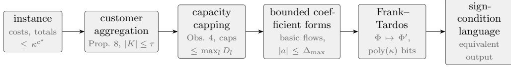
Figure 7: The compression pipeline of Proposition 9. Aggregation and capping (Prop. 8, Obs. 4) bound the entities and the numeric entries by \text{poly}(\kappa) , total unimodularity of the oracle networks of Proposition 1 turns acceptance into sign conditions on integer forms with coefficients of magnitude at most \Delta_{\max} , and the Frank–Tardos step replaces the cost vector \Phi by an equivalent \Phi' of \text{poly}(\kappa) bits, so the bounded subclass compresses in \kappa .
