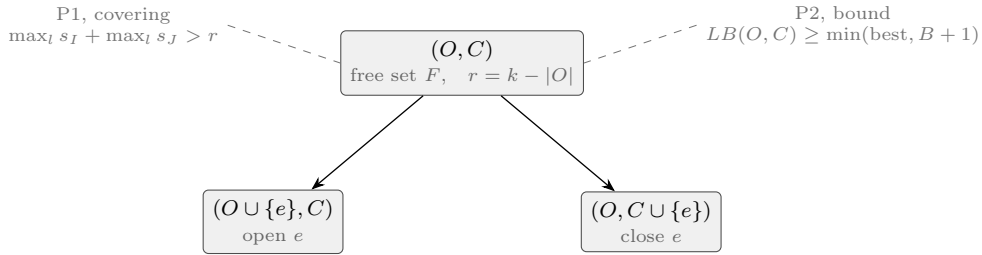
Figure 4 One branching step of Algorithm 1. A node carries the forced-open set O , the forced-closed set C , the free set F and the remaining cardinality r , and branching on a free facility e produces the two children along the solid arrows. The dashed leaders attach P1 and P2 to the popped node they test, while P3 fires only at a leaf, so the three prunes act exactly on the named quantities (Lemma 1, Proposition 6).
