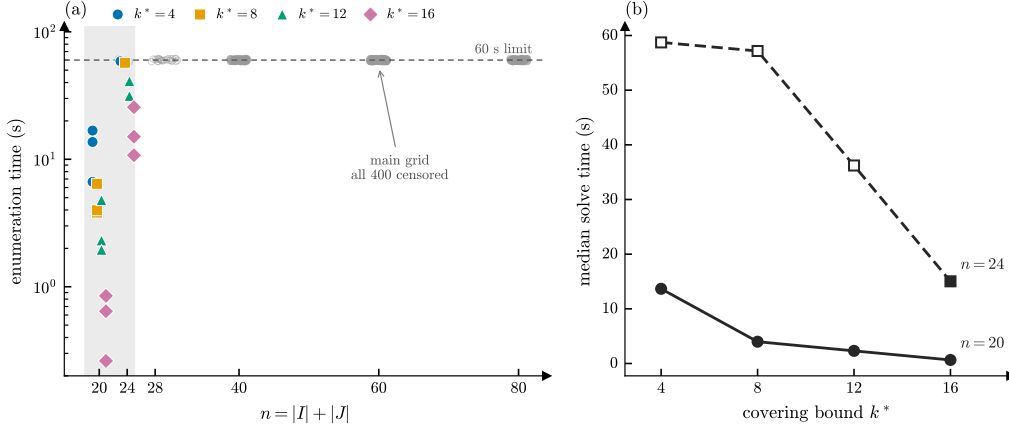
Figure 9: The enumeration algorithm on the controlled family, all 460 runs under the 60 s limit. Panel (a) plots time against n = |I| + |J| . Solved runs are filled and coloured by the covering bound k^* , and they occur only in the shaded band up to n \approx 24 . Every run beyond it is censored, shown as grey open circles on the limit line, including the whole 400-instance main grid, which lies at n \geq 40 . Panel (b) gives the median solve time against k^* at n = 20 and n = 24 , where instances with a larger bound solve faster, with medians taken over solved runs only. Open markers in panel (b) are medians over fewer than three solved runs. Lower is better in both panels, and the censored band beyond n \approx 24 is the observed border of the regime that Theorem 8 delimits.
