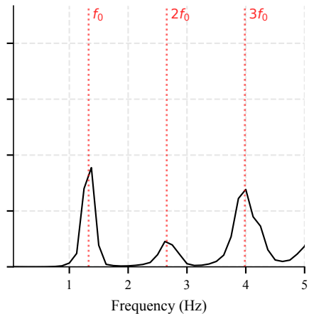
(c) Standing (HR = 79.7 bpm, f_0 = 1.33 Hz)
