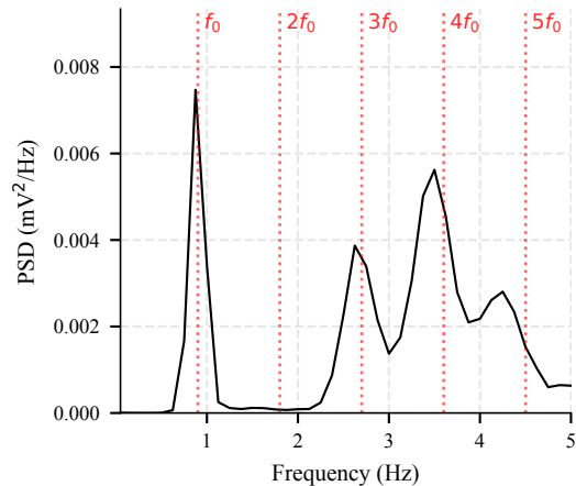
(a) Supine (HR = 54.0 bpm, f_0 = 0.90 Hz)
