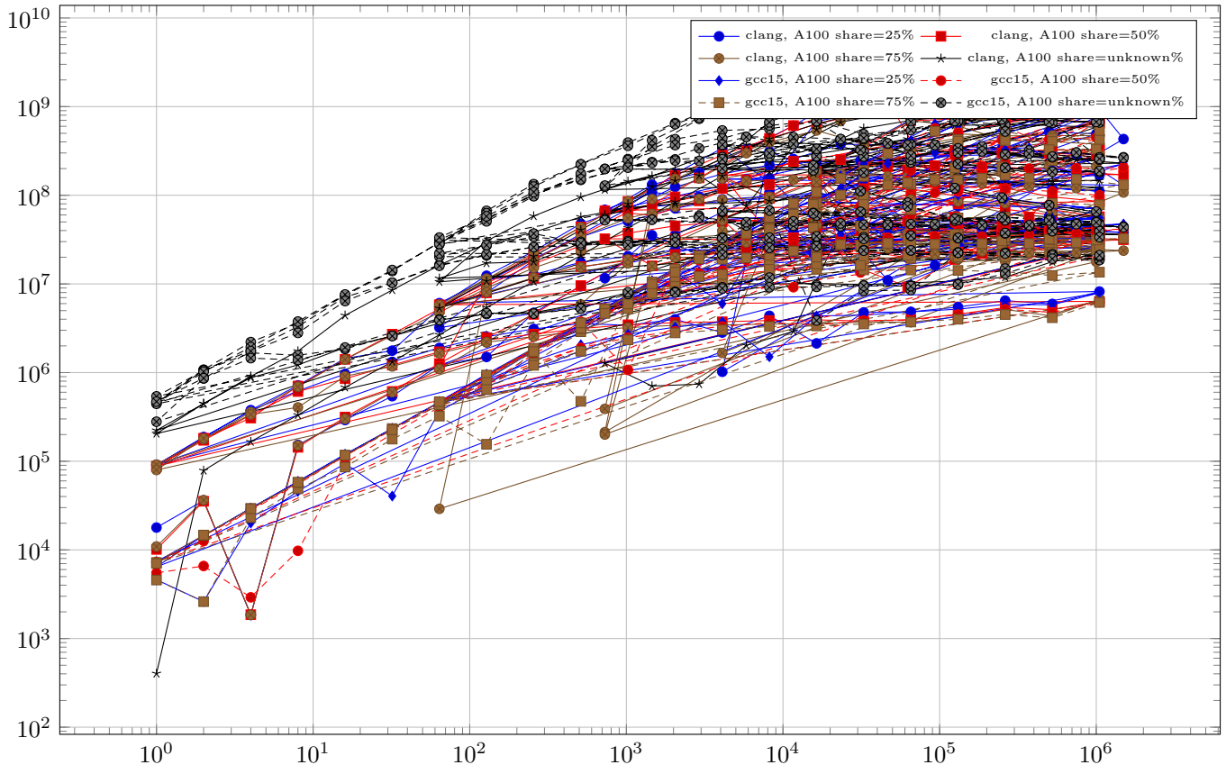
range-benchmark-sol-6d – K3 mixed OpenMP
