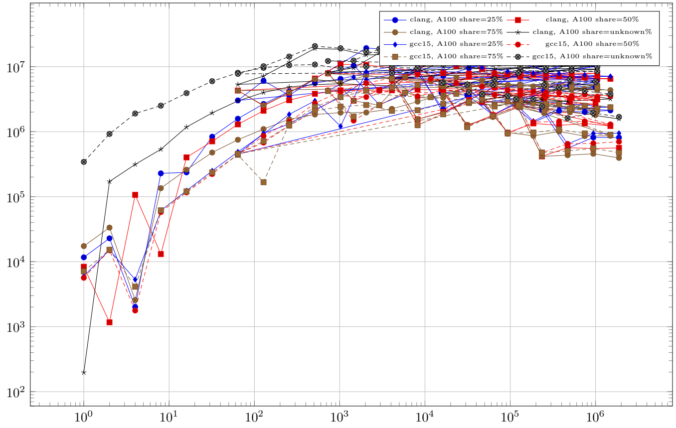
range-benchmark-advection-6d – K3 mixed OpenMP
