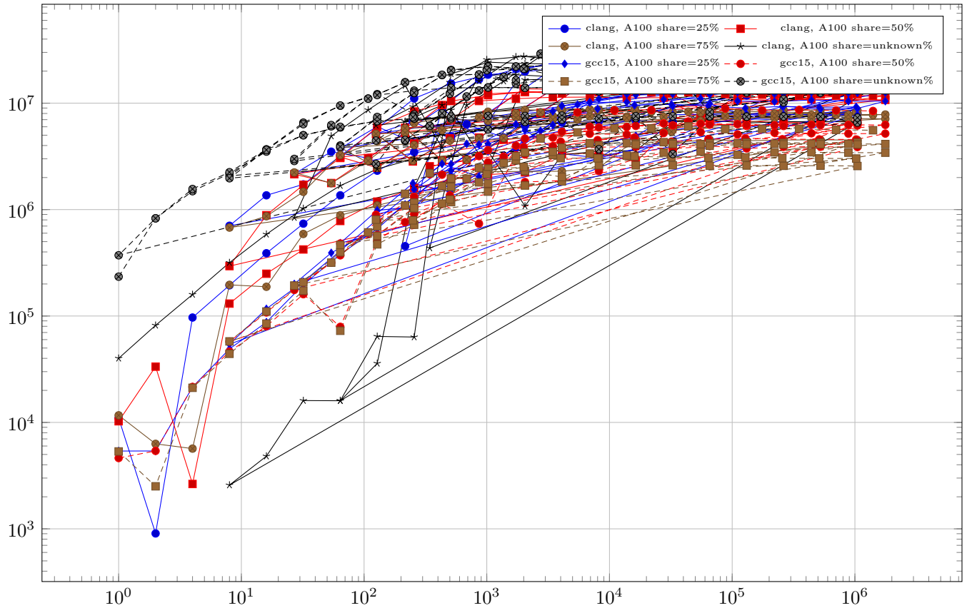
range-benchmark-advection-3d – K3 mixed OpenMP
