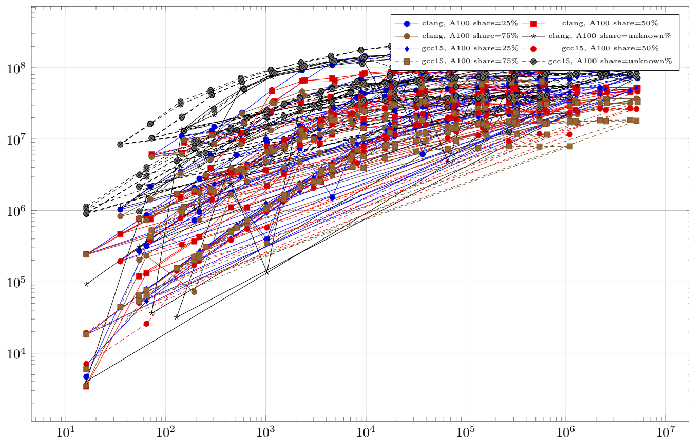
range-benchmark-advection-p-adaptivity-3d – K3 mixed OpenMP
