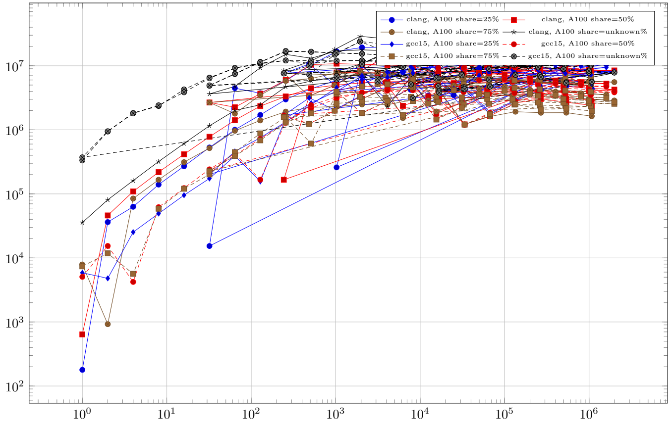
range-benchmark-advection-5d – K3 mixed OpenMP
