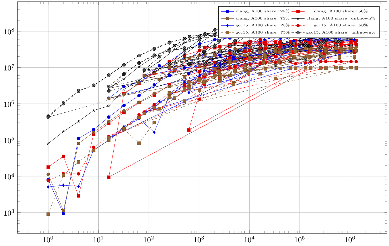
range-benchmark-mass-4d – K3 mixed OpenMP
