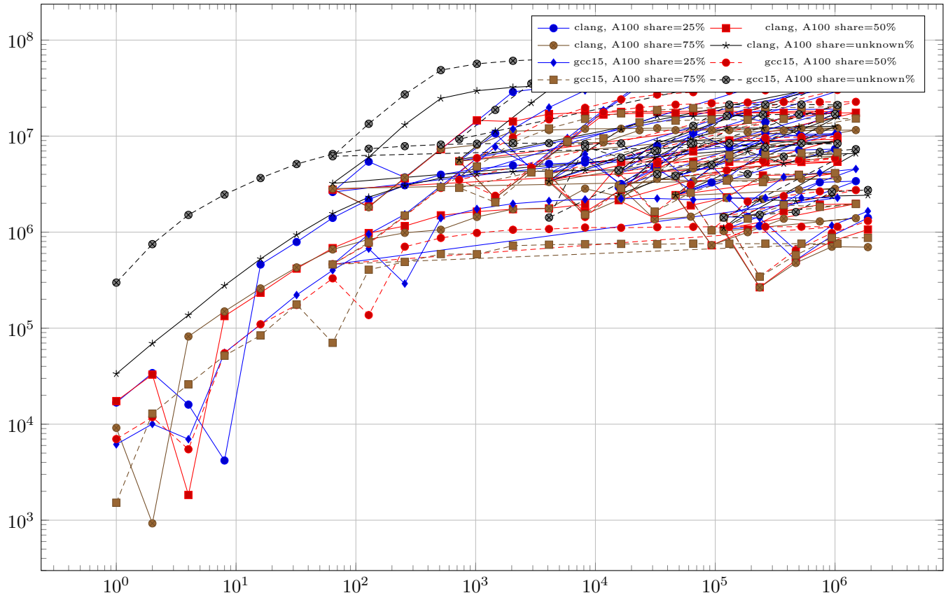
range-benchmark-mass-6d – K3 mixed OpenMP
