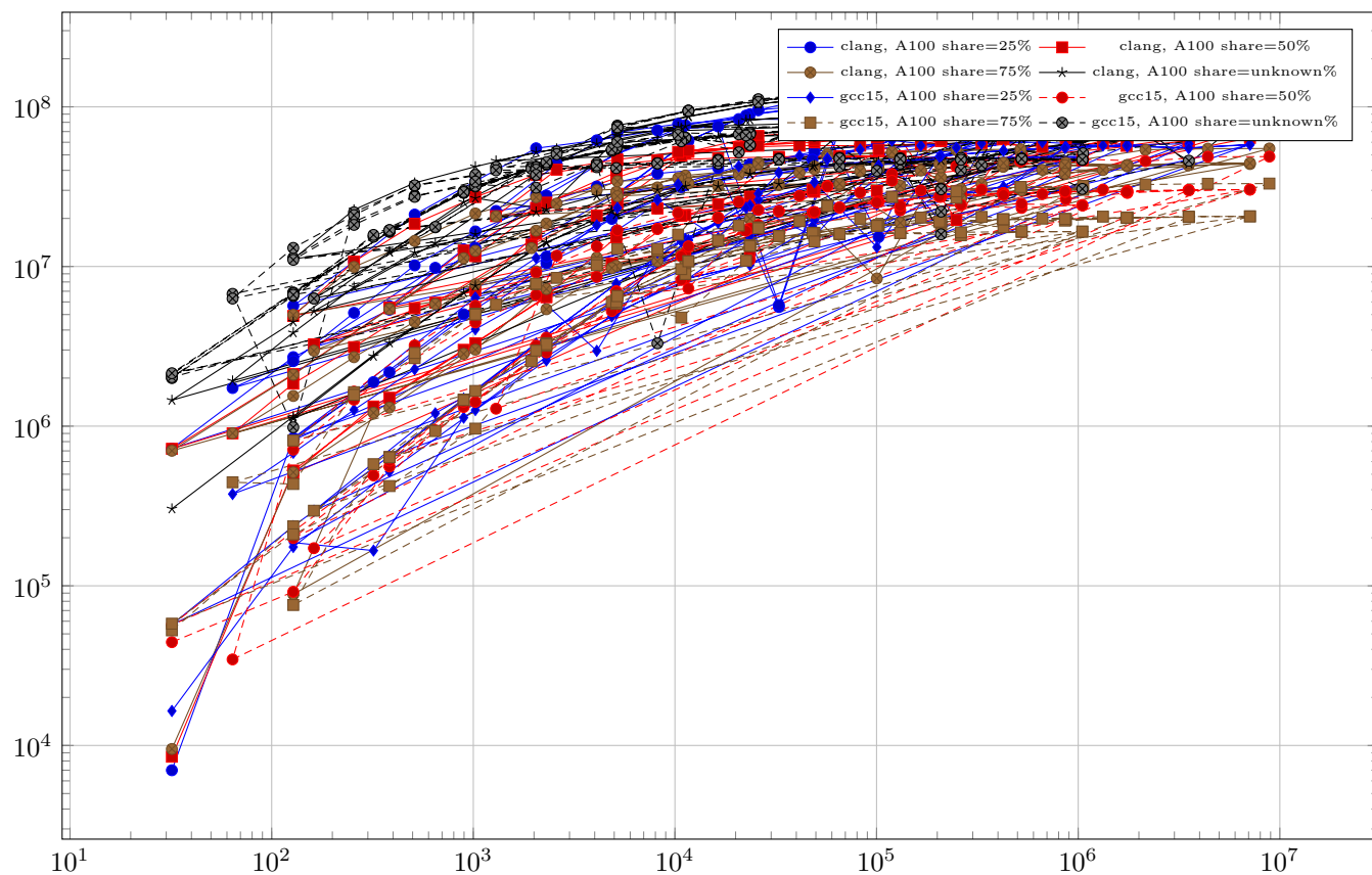
range-benchmark-advection-h-adaptivity-4d – K3 mixed OpenMP
