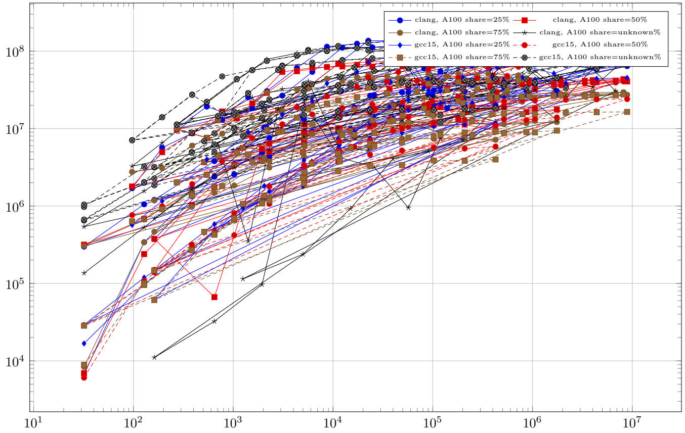
range-benchmark-advection-p-adaptivity-4d – K3 mixed OpenMP
