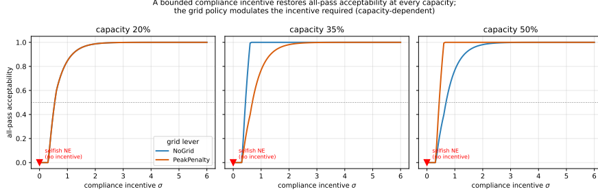
Figure 12: All-pass acceptability of the induced driver equilibrium as a function of the compliance incentive \sigma , for the two grid policies at each capacity. The selfish equilibrium ( \sigma = 0 , red marker) is unacceptable; a bounded incentive restores all-pass at every capacity. The grid policy modulates the incentive required, with a capacity-dependent sign (GridPeakPenalty helps at 50% capacity).
