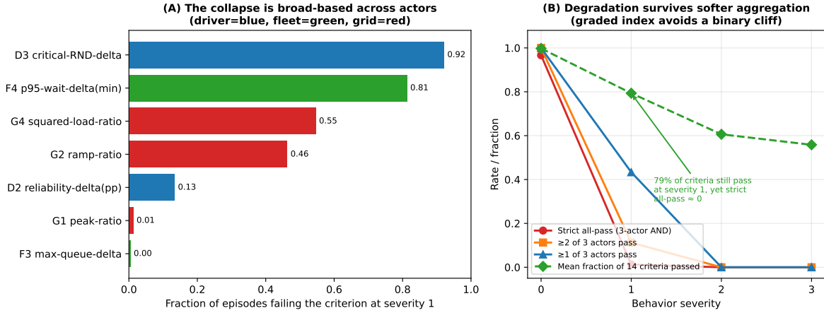
Figure 9: Robustness of the acceptability definition. (A) Fraction of severity-1 episodes failing each binding sub-criterion, coloured by actor (driver, fleet, grid); the collapse is driven by four distinct criteria across all three actors, not a single tight gate. (B) Acceptability rate under alternative aggregation logics and the graded fraction-of-criteria index; the degradation survives softer aggregation, while the graded index (about 0.79 of criteria still passing at severity 1) avoids overstating a binary cliff. Twenty-seed service-oriented family.
