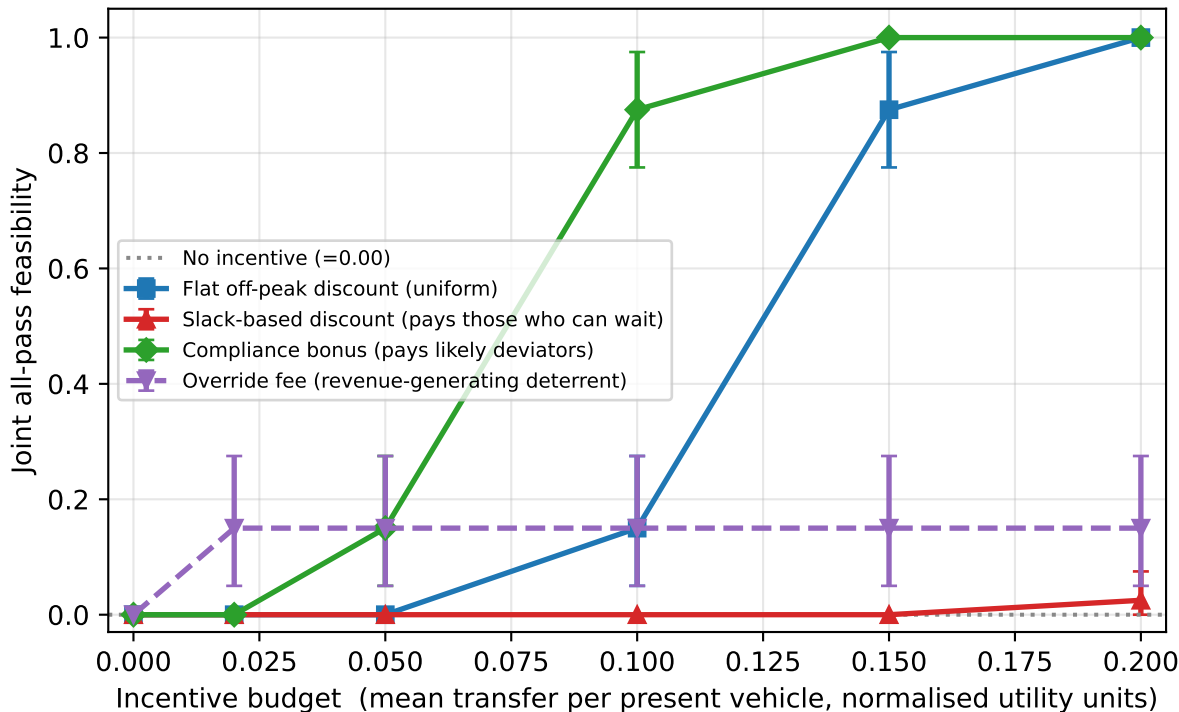
equal-budget incentive comparison (5% deviation, 35% capacity; 20 seeds, 95
