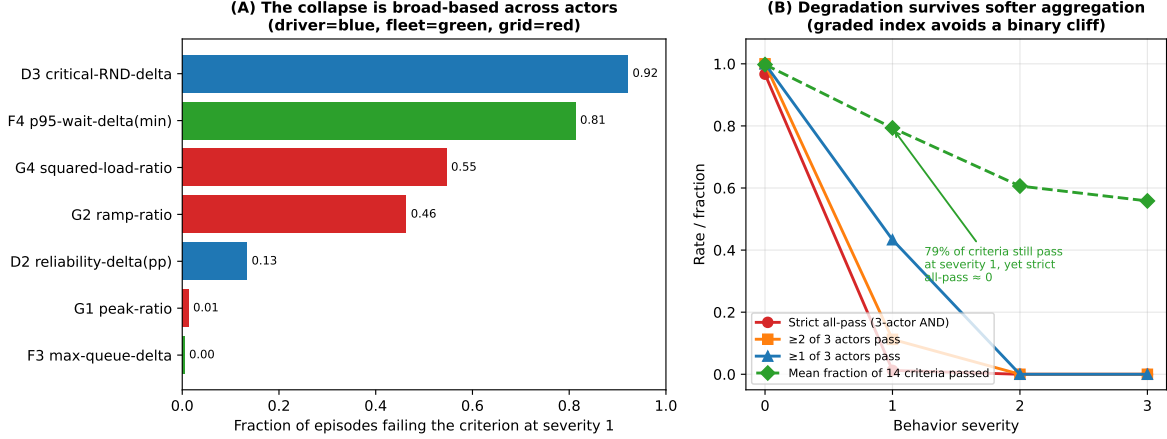
Figure 9: Robustness of the acceptability definition. (A) Fraction of severity-1 episodes failing each binding sub-criterion, coloured by actor; the collapse is driven by four distinct criteria across all three actors, not a single tight gate. (B) Acceptability rate under alternative aggregation logics and the graded fraction-of-criteria index; the degradation survives softer aggregation, while the graded index ( \approx 0.79 of criteria still passing at severity 1) avoids overstating a binary cliff. Twenty-seed service-oriented family.
