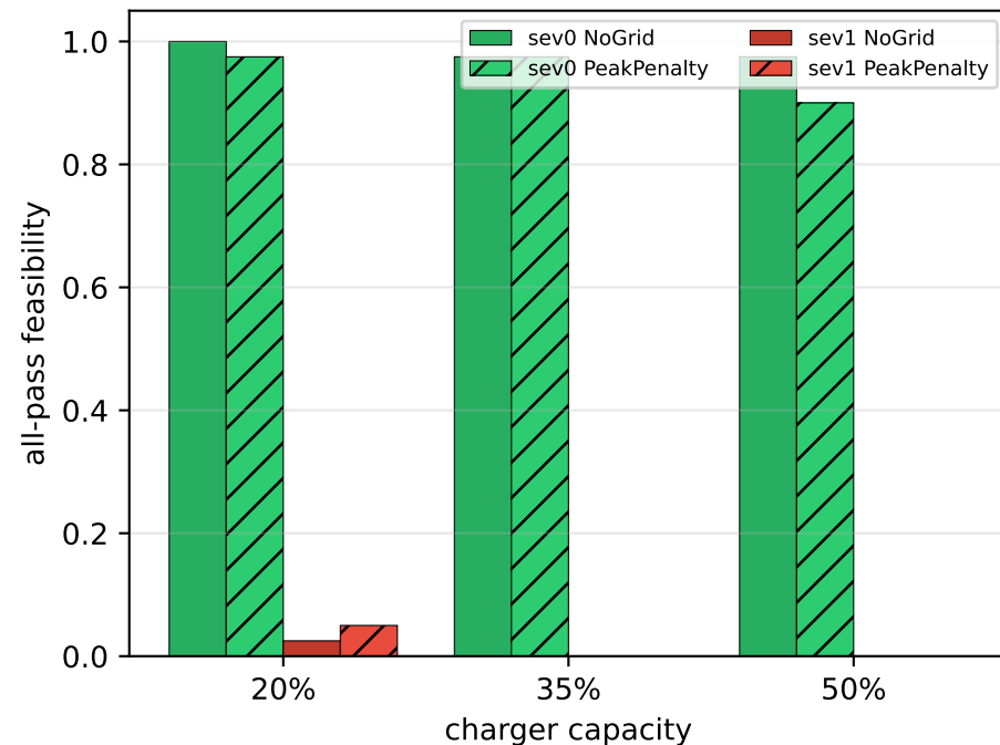
(A) Collapse is uniform across capacity (more chargers do not help)
