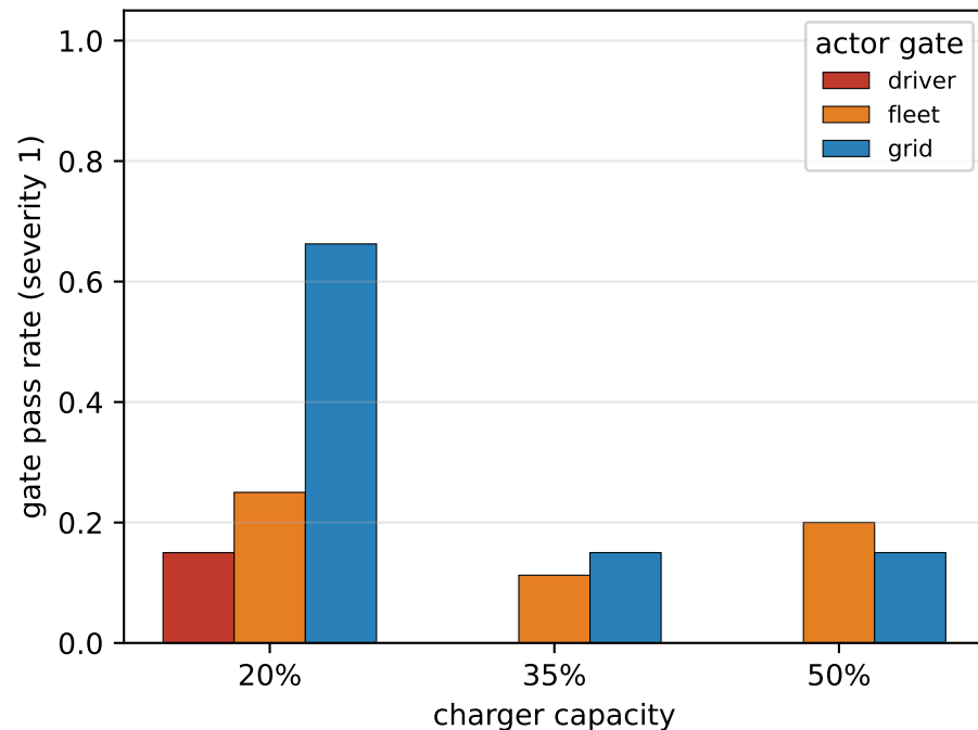
(B) The driver gate binds first (lowest-passing actor across capacity)
