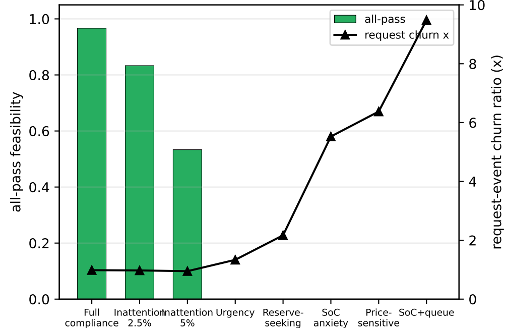
(C) Self-service behaviors (high churn) collapse it; inattention (low churn) does not
