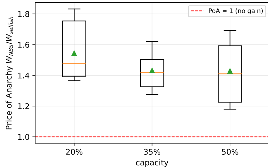
PoA across 243 game-parameter configs per capacity (always > 1)
